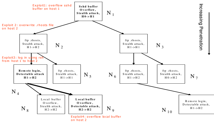
Fig. 6. Example Sub-Attack Graph from Fig. 1
