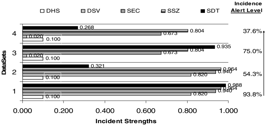
Fig. 7. Alert Situation for Host 'mill'
