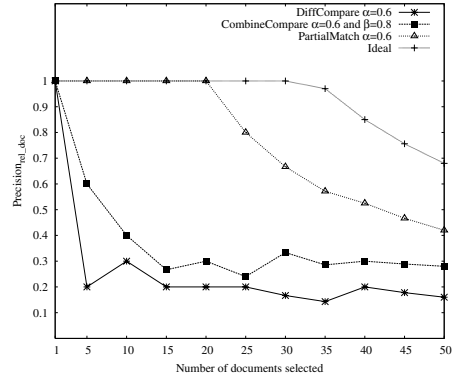
(f) Document selection precision(AEB-1000)
