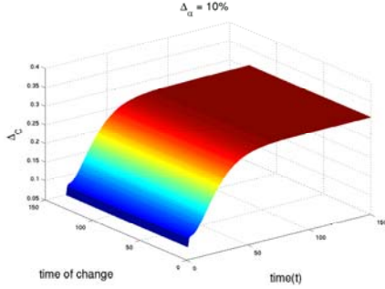
Fig. 7. Sensitivity of the safe queue with respect to a 10% change in the \alpha parameter at different time stamps
