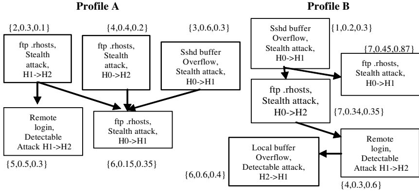
Fig. 2. Attack paths based on profiles from Fig. 1 (3 Tuple{Cost, Skill, Tenacity})
