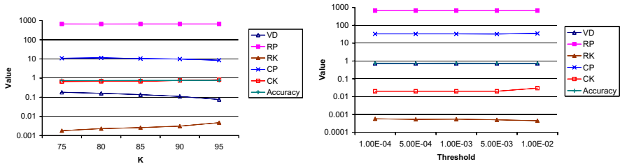
(a) The influence of k in SVD (b) The influence of threshold \epsilon
