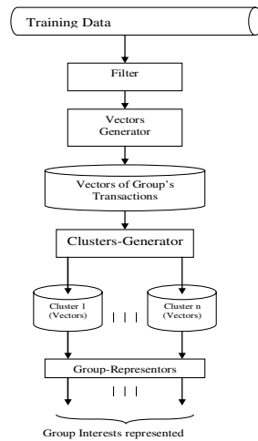
Fig. 1. The Learning phase of the model
