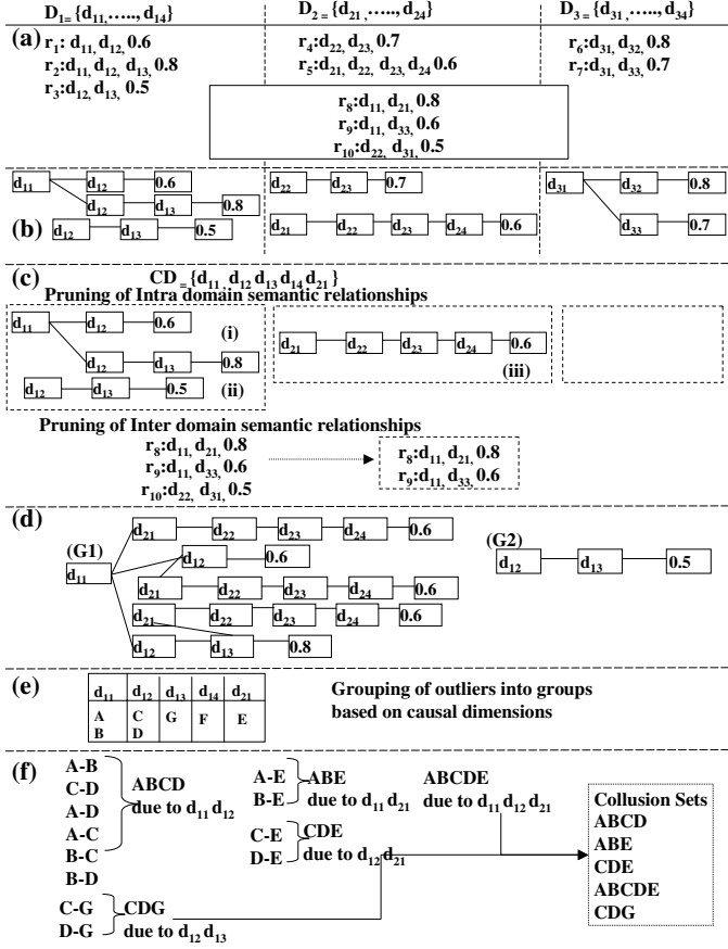
Fig. 1. An example depicting the collusion set detection steps
