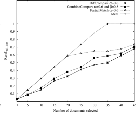
(b) Document selection recall (AEB)
