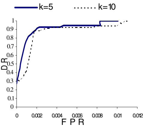
Fig. 1. ROC curve for the S^3M scheme at k=5,10
