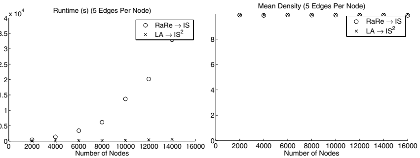
Fig. 4. Runtime and performance of the previous algorithm (RaRe followed by IS) and the current algorithm (LA followed by IS 2 ) for preferential attachment graphs
