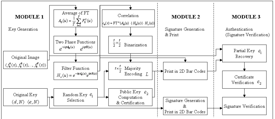
Fig. 6. Block Diagram of Phase 2 System
