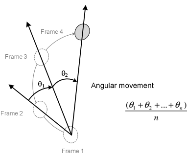
Fig. 10. Angular Movement Feature
