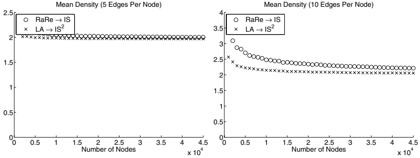
Fig. 3. Performance (average density) of the algorithm compared to the previous algorithm
